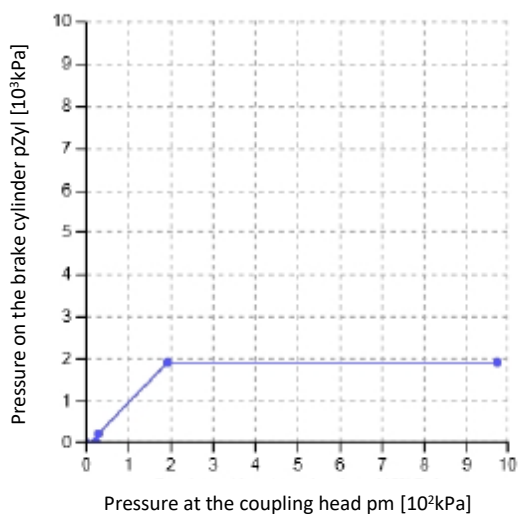
Control with a manual controller (pressure limitation)
