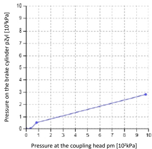
Control with BPW MLB (proportional pressure control)
